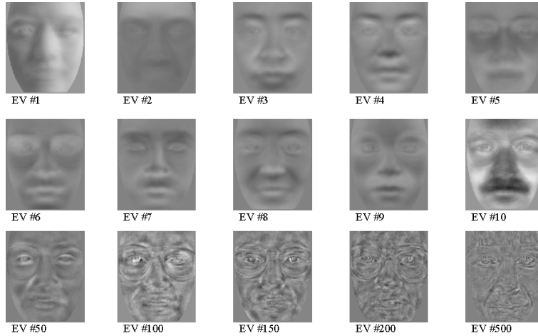
Figure 2: Eigenvectors 1-10, 50, 100, 150, 200 and 500
